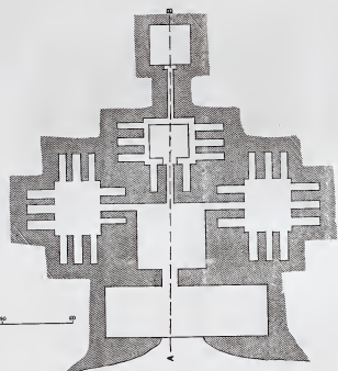
PLAN OF A REMARKABLE TOMB ON THE WESTERN SIDE OF THE KEDRON SOUTH OF BIR EYUB ABOUT 1/4 MILE.
